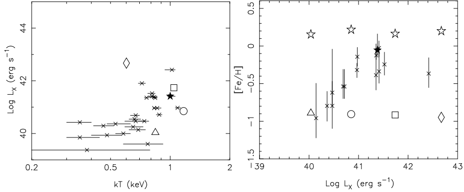
Figure 1: Comparison of the simulated and observed (crosses with error bars) L_X - T_X relations ( left panel ) and [\text{Fe}/\text{H}]_X - L_X relations ( right panel ). The circle/square/diamond/triangle indicates the predictions of Model 1/2/3/4. Open stars in the right panel show the predicted mean metallicity of the stellar component for the four models. The observational data are from Matsushita, Ohashi & Makishima (2000). The solid star presents the position of NGC 4472.
