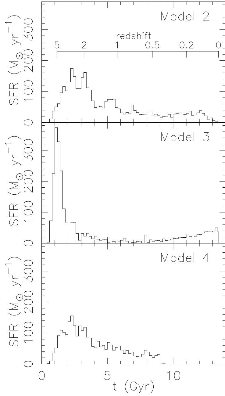
Figure 3: Time variation of the star formation rate for Models 2 (upper), 3 (middle), and 4 (lower).
