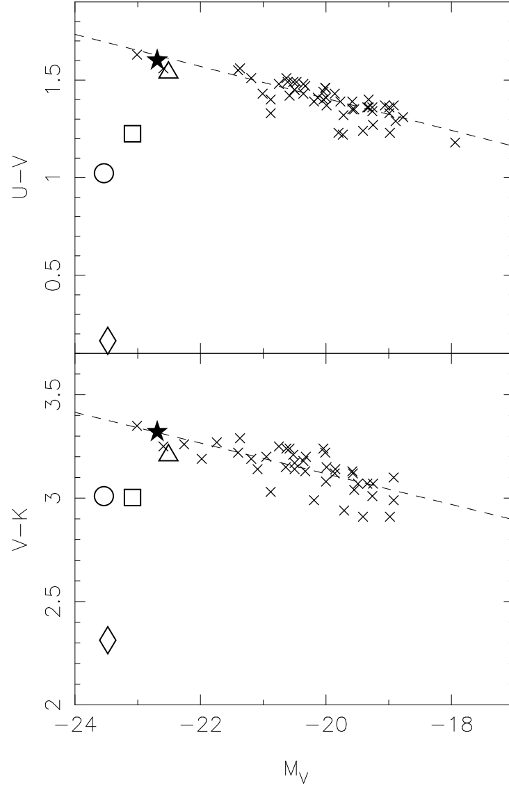
Figure 2: Comparison of the simulated U - V and V - K CMRs (circle/square/diamond/triangle for Model 1/2/3/4) and those of the Coma cluster ellipticals (crosses). The observational data are from Bower, Lucey & Ellis (1992). The dashed line shows the CMR fitted to the Coma Cluster galaxies. The solid star shows the position of NGC 4472.
