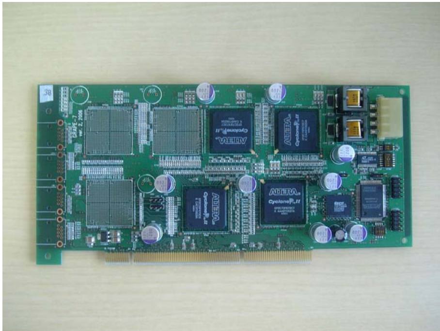
図 4.5: GRAPE-7 model 300
